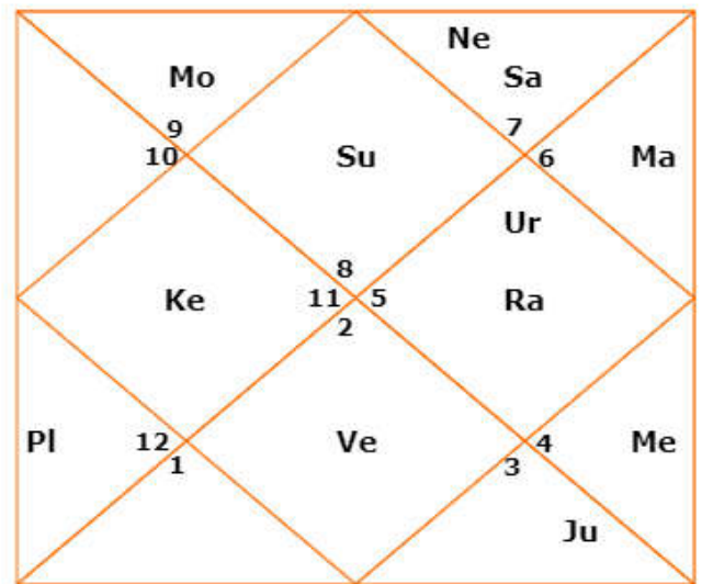
Navamsa Chart
