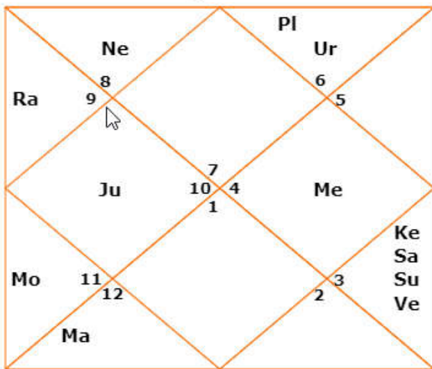
Lagna Chart
